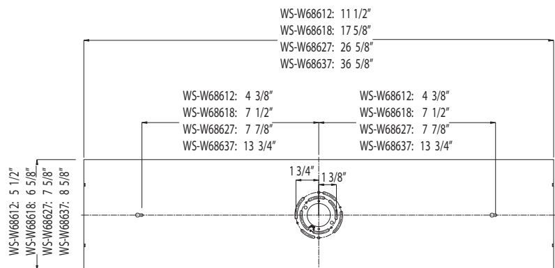
Mounting Back Plate Dimensions
