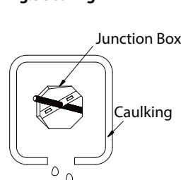
Fig.3 Sealing
