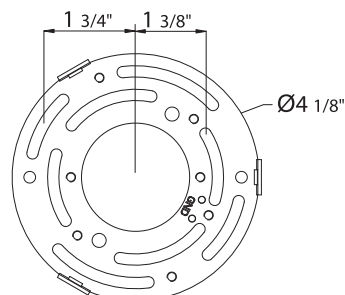
WS-53318 Mounting Back Plate
