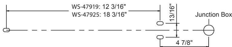
Fig.4 Installation Location
