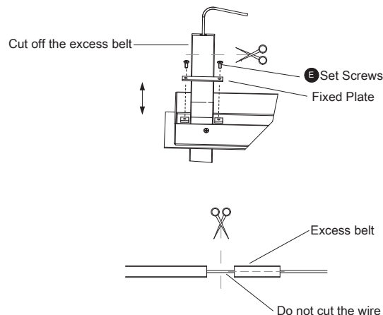
Fig. 5 Belt adjustment
