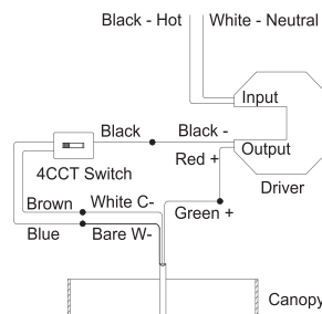
Fig. 4 Driver Wires
