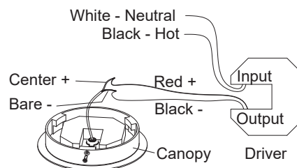
Fig.3 Driver Wires
