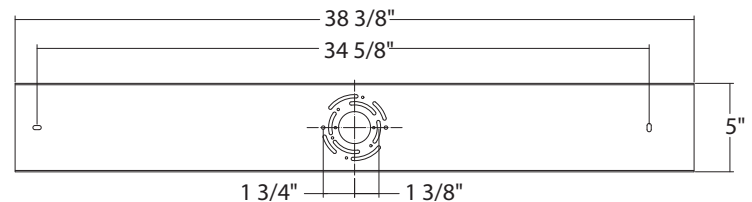
Mounting back plate
