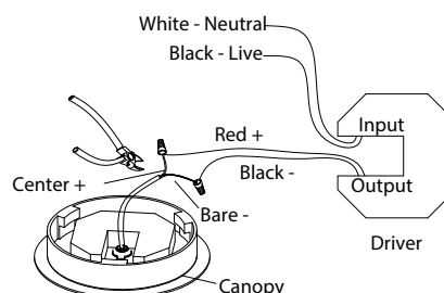
Fig.3 Driver Wires
