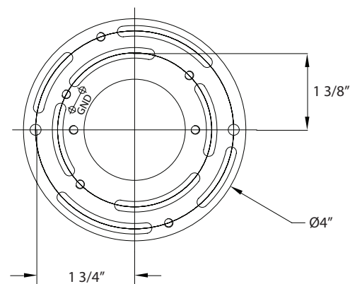
Back Plate Dimensions
