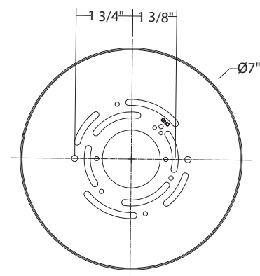
Mounting Back Plate
